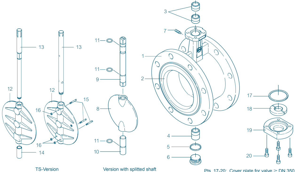
Pts. 17-20: Cover plate for valve ≥ DN 350
